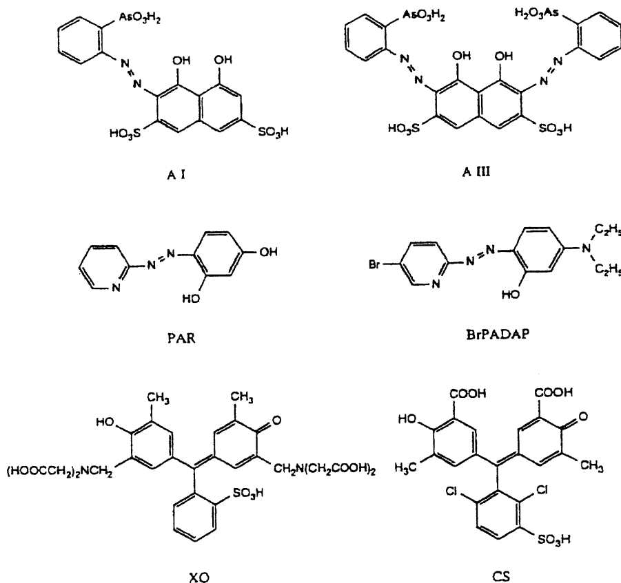
Fig. 10. Structures of six metallochromic ligands discussed by Haddad and co-workers in [130].
