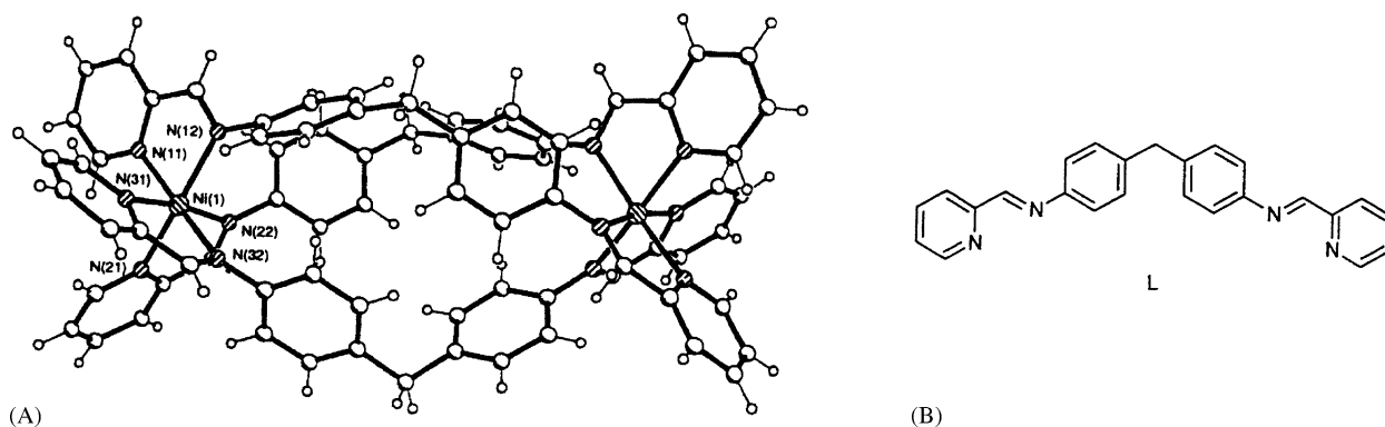
Fig. 23. One enantiomer of the chiral supramolecular helicate complexes, [M^{II}_2L_3] , M^{II} = Fe^{II} or Ni^{II} , that binds to cellulose (reproduced from [360] with permission of the copyright holders).
